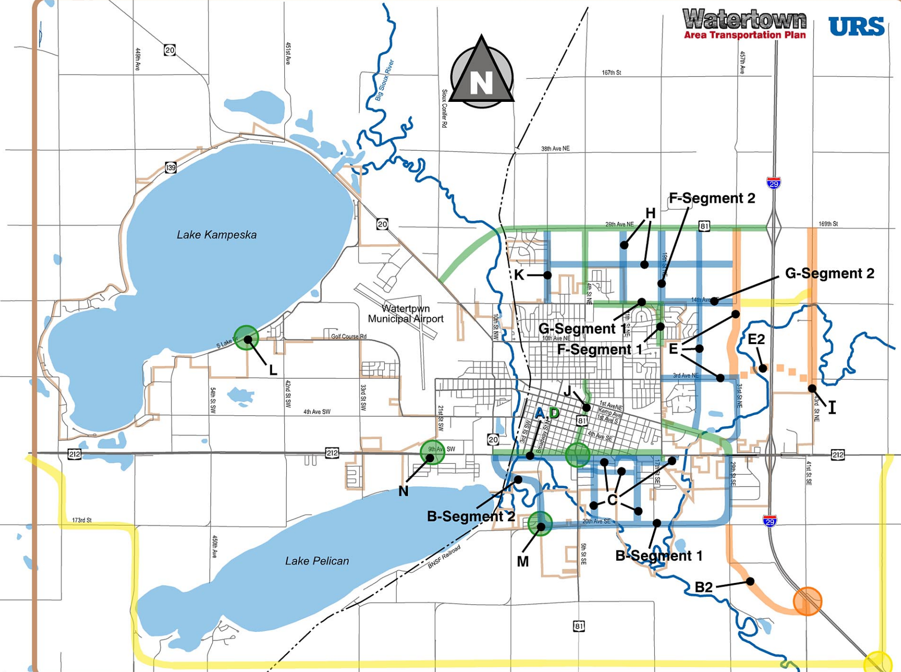
Phasing of Recommended Roadway Projects
